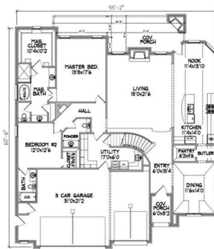
A Lower Level Floor Plan
